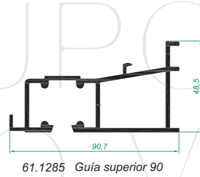
61.1285 Guía superior 90
