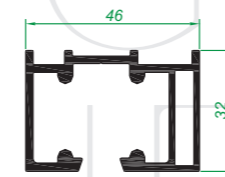
61.1246 Guía Sup. 46
