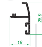
61.6600 Acople cierre
