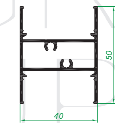
61.810 Transversal Lamas
